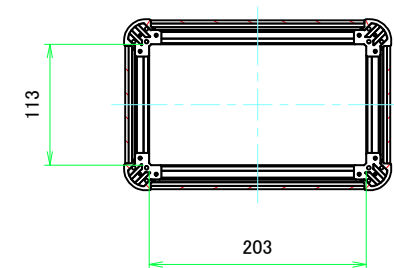
C-C (1:5)
